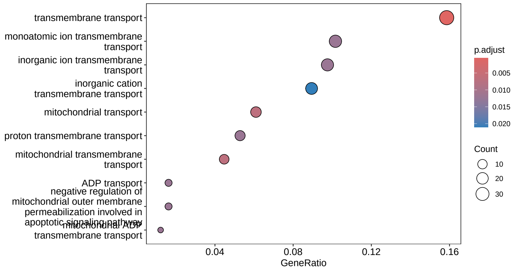
up_200uM_only: GO BP (simplified)
